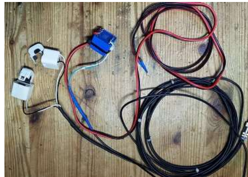
Transformers and wire harness example
